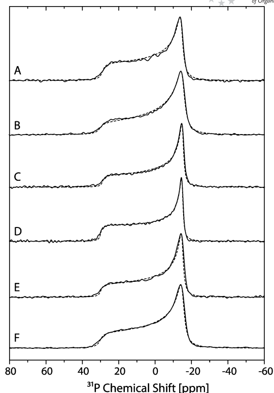
Figure 2. 31 P NMR spectra of POPC membranes in the presence of 20 mol-% 7/8 (A), 15 (B), 19 (C), 11 (D), 27 (E), and of pure POPC membranes as the reference (F). The measurements were conducted at a water content of 40 wt.-% and a temperature of 30 °C. The dashed lines represent best-fit simulations of the 31 P NMR spectra.
