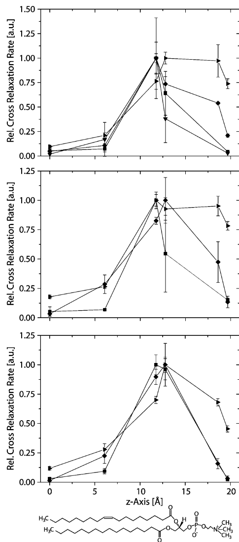
Figure 5. Relative ^1\text{H} NOESY cross-relaxation rates between the nucleoside moiety of (7/8) ( \blacklozenge ), 11 ( \blacktriangle ), 15 ( \blacksquare ), and 19 ( \blacktriangledown ) and segments of the POPC molecules within the membrane as a function of the coordinates of such lipid segments. Localization of 6-H (top) and 5-H (middle) of the uracil nucleobase and of 1'-H of the ribose with respect to the membrane normal is shown. The approximate localization of these hydrogen atoms with respect to various segments of the lipid molecules in the host membrane can be estimated from the phospholipid molecule drawn below. The measurements were carried out at a 1:4 molar ratio of lipophilic nucleoside/POPC and at a temperature of 30 °C.
