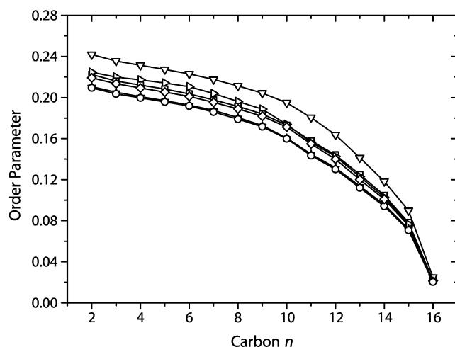
Figure 3. Smoothed order parameter profiles obtained from ^2\text{H} NMR spectra of [\text{D}_{31}]\text{POPC} of the samples [\text{D}_{31}]\text{POPC} (○), (7/8)/ [\text{D}_{31}]\text{POPC} (◊), 11/ [\text{D}_{31}]\text{POPC} (◐), 15/ [\text{D}_{31}]\text{POPC} (◑), 19/ [\text{D}_{31}]\text{POPC} (▽), and 27/ [\text{D}_{31}]\text{POPC} (*) all at a molar ratio of 1:4 and a temperature of 30 °C.
