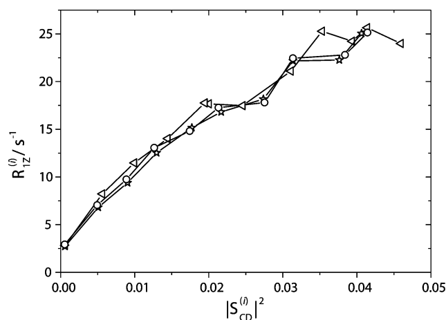
Figure 4. Dependence of the longitudinal relaxation rate R_{1Z}^{(i)} on the corresponding order parameter squared for 27/ [\text{D}_{31}]\text{POPC} (*) and 28/POPC (◐) at a molar ratio of 1:4, and for pure [\text{D}_{31}]\text{POPC} (○) at 40 wt.-% \text{H}_2\text{O} and a temperature of 30 °C. The elastic properties of the [\text{D}_{31}]\text{POPC} membranes are unchanged in the presence of the lipophilic nucleoside 27 indicating that this molecule is well incorporated into the bilayer without interfering with the elastic properties of the membrane. This is also seen from the square-law plot of deuteriated 28 which is essentially identical to POPC in the presence and in the absence of 27.
