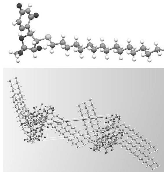
Figure 1. X-ray crystal structure of 2'-hexadecylthio-2'-deoxyuridine ( 27 ). The upper structure shows the single molecule and the lower panel depicts the molecular assembly in the crystal.
